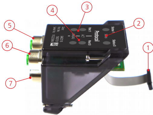
Figure 2: Overview electrical components of the exchangeable cover with Industrial Ethernet
