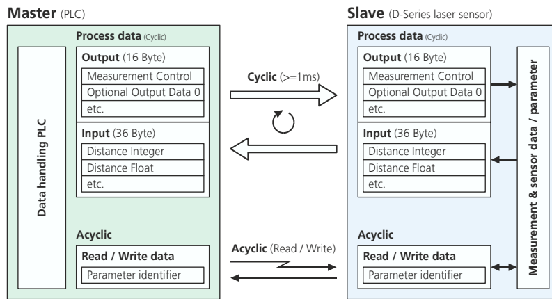
Figure 8: Cyclic (Process data) and acyclic communication between Industrial Ethernet Master (PLC) and the D-Series device with Industrial Ethernet interface.
