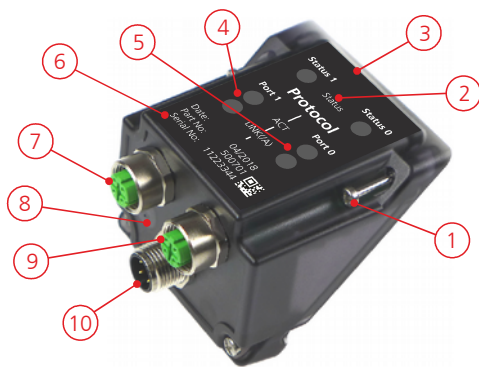
Figure 1: Components with detail information of the exchangeable cover with Industrial Ethernet
