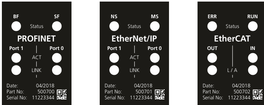
Figure 12: Labeling of the available exchangeable cover with Industrial Ethernet.
