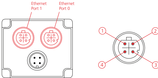
Figure 4: Connection diagram of the Ethernet port 0 & 1
