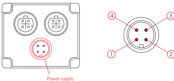
Figure 3: Connection diagram of the sensor power supply
