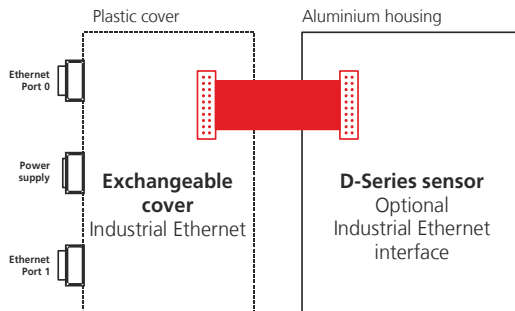
Figure 5: Connection diagram of exchangeable cover with Industrial Ethernet and D-Series sensor
