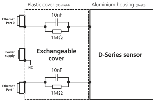
Figure 6: Shielding concept of the D-Series sensor and the exchangeable cover with Industrial Ethernet
