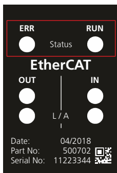
Figure 11: EtherCAT® status LED's
